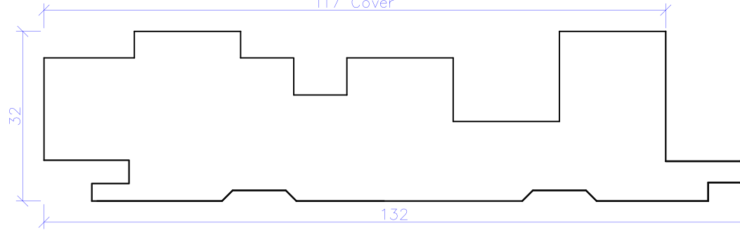
Profile C3
