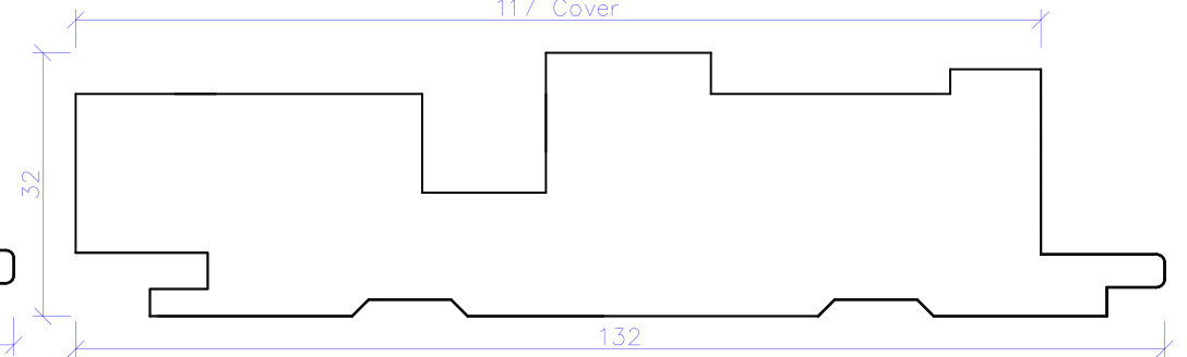
Profile C4
